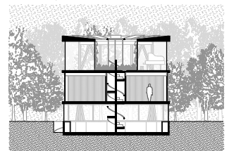
Section: The three levels of the house and the relation with the context
