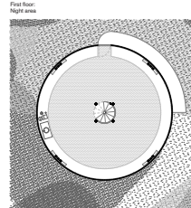
Ground floor plan: Entrance and living area
