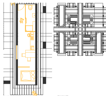
Floor plan tiny houses 1:25
